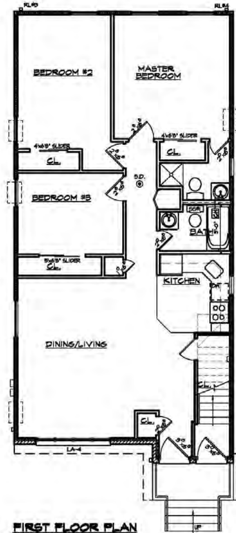
FIRST FLOOR PLAN SCALE: 1/8"=1'-0"
